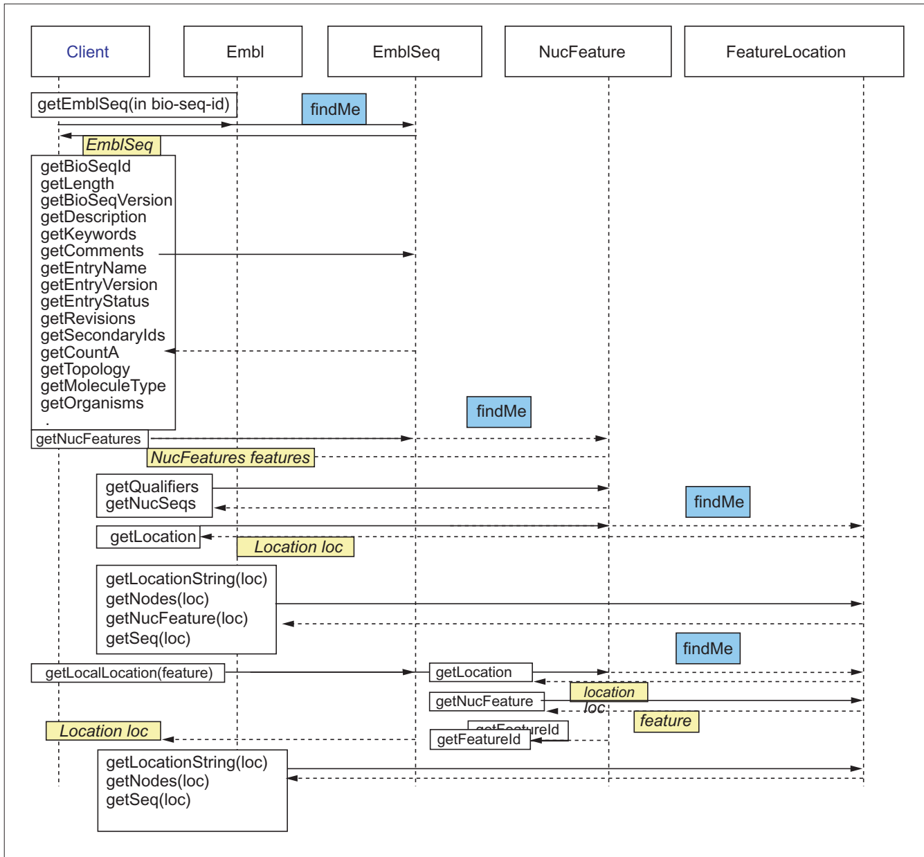
Figure 10 Access to the EMBL database via the CORBA server. The client submits its query with bio-seq-id to the Embl object, which is a factory object representing the whole database. It invokes the operation findMe provided by EmblSeq object, which in turn invokes the loader object. The EmblSeq reference is returned to the client. Once the client has the EmblSeq object reference, it can then invoke the methods provided by EmblSeq to get the sequence information defined in SeqInfo . The object attributes are obtained through invoking the methods. Further queries can be made through the invocation to other methods.
